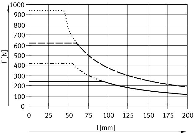
DFM-32 ... 63-GF, Hub 80 ... 100 mm
