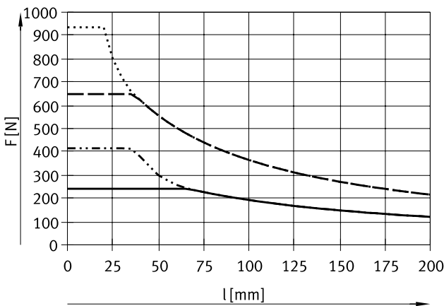
DFM-32 ... 63-KF, Hub 80 ... 100 mm
