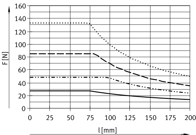
DFM-12 ... 25-KF, Hub 40 ... 100 mm
