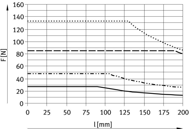
DFM-12 ... 25-GF, Hub 40 ... 100 mm
